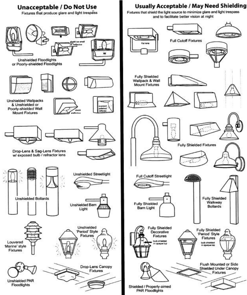
Figure C: The lights on the left are nonconforming. Those on the right can be used in most cases. However, the mounting height and proximity to the property line may cause the lights to need additional shielding to prevent the luminous elements from being visible from any other property.
